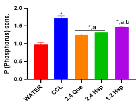
Figure 1. Effect of quercetin and hesperidin pretreatment on CCL4 mediated decrease in kidney function test (a) Na (b) K (c) Cl (d) Ca (e)P. Bar represents mean ± SEM (n=5). Bar with different letters is significantly different at P < 0.05
