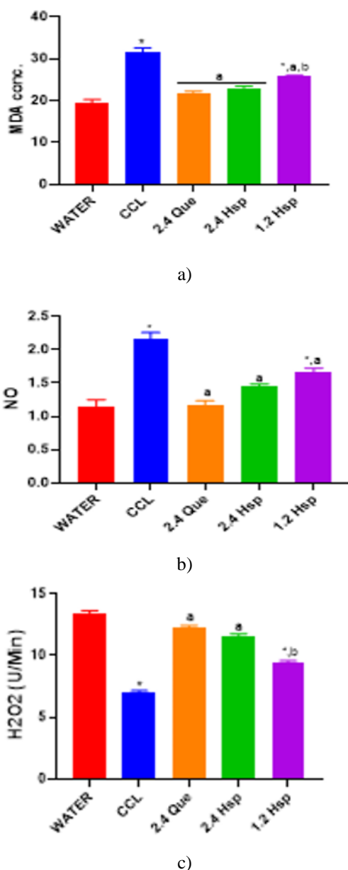
Figure 2. Quercetin and hesperidin pretreatment effects on CCL4 mediated increase in oxidative stress markers in rats on kidney parameters. (a) MDA level (b) Nitric oxide (c) Hydrogen peroxide. Bars represent mean \pm SEM ( n=5 ). Bars with different letters are significantly different at P < 0.05 .
