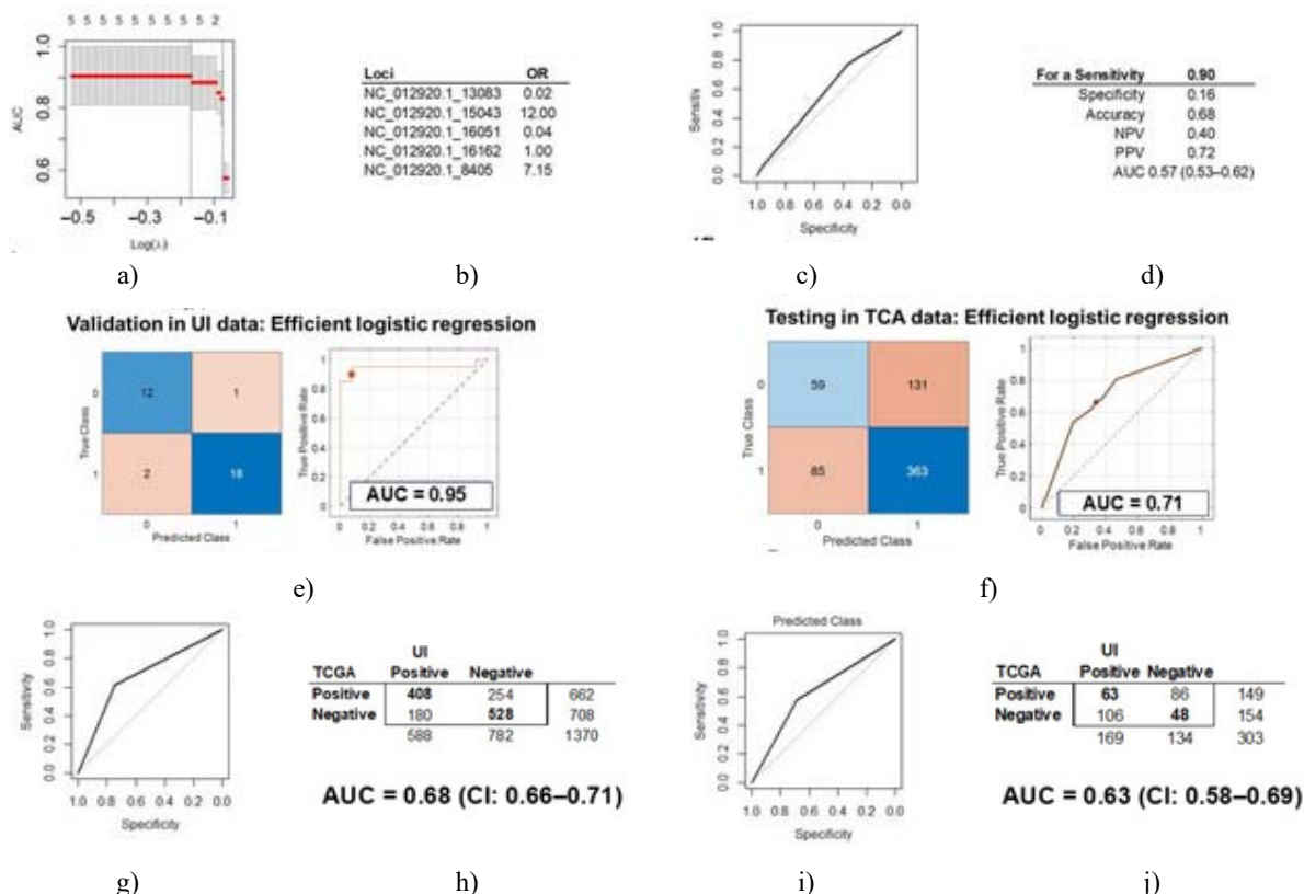
Figure 4. Model training, validation, and testing. (a) The LASSO model for predicting HGSC was validated on UI data using only five key mtDNA variants, achieving an AUC of 91% (CI: 82–100%). (b) The odds ratios of variants in the LASSO model indicate increased risk for HGSC when OR >1 and protective effects when OR <1. (c) ROC curve of the model tested on TCGA data using the pROC package. (d) Model performance on TCGA data, optimized for 0.9 sensitivity, reached an AUC of 0.57 (CI: 0.53–0.62). (e) Validation in UI data with MATLAB, using efficient logistic regression, shows the confusion matrix (left) and ROC curve (right), yielding an AUC of 0.95. (f) Testing on TCGA data produced a confusion matrix (left) and ROC curve (right) with an AUC of 0.71. (g) Correlation analysis of the MT-CYB variant with differential gene expression in HGSC versus controls indicated moderate agreement between UI and TCGA data (AUC = 0.68, CI: 0.66–0.71). (h) A 2 × 2 matrix from Figure 4g illustrates that 1370 genes were shared between UI and TCGA datasets. (i) Correlation of MT-CYB expression with gene expression revealed moderate concordance between the datasets (AUC = 0.63, CI: 0.58–0.69). (j) The 2 × 2 matrix for Figure 4i shows 303 genes common to both datasets.
