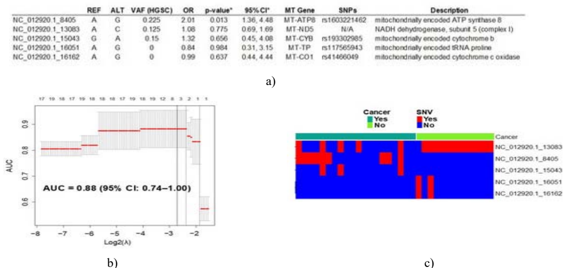
Figure 1. Prediction of HGSC based on mtDNA alterations. (a) Out of 393 identified mtDNA variants, five were selected as the most informative for predicting ovarian cancer, achieving an AUC of 0.88 (95% CI: 0.74–1.00). REF indicates the reference allele; ALT represents the alternative allele detected; VAF denotes the variant allele frequency in cancer samples; OR reflects the odds ratio comparing alleles in cancer versus control samples; MT Gene specifies the mitochondrial gene name; SNP refers to the known single nucleotide polymorphism identifier. *The LASSO regression approach prioritizes predictive variable selection rather than formal statistical inference; variant effect sizes and confidence intervals were estimated using the R package selectiveInference (v. 1.2.5), though potential overfitting may influence results. (b) Visualization of LASSO regression with 95% confidence intervals: the top axis shows the number of SNVs selected by the model, the left axis indicates the corresponding AUC, and the bottom axis depicts the log 2 -transformed lambda tuning parameter chosen through bootstrapping and cross-validation. Dotted lines indicate reference lambda values: lambda.1se (right), lambda.min (center), and the selected λ (left). (c) Heatmap of mtDNA variants included in the model per sample, with red representing variant presence and blue indicating absence; N/A indicates not applicable.
